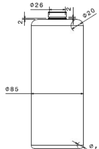
Front view Scale: 1:2
